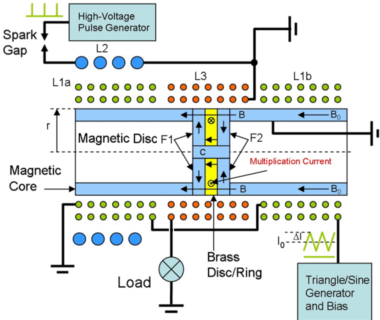
Fig.1 Cross-section of the example coil. Some of the actual implementation details may differ from the arrangement shown above, but that will not alter the operation of device. This diagram is not to scale.
