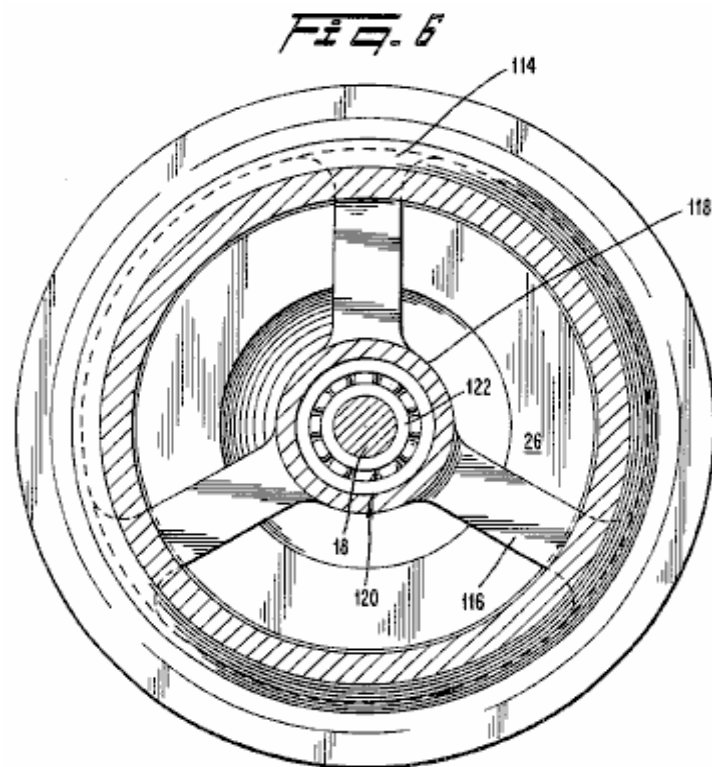
Fig.6 is a cross-sectional view taken along line 6--6 in Fig.1;
