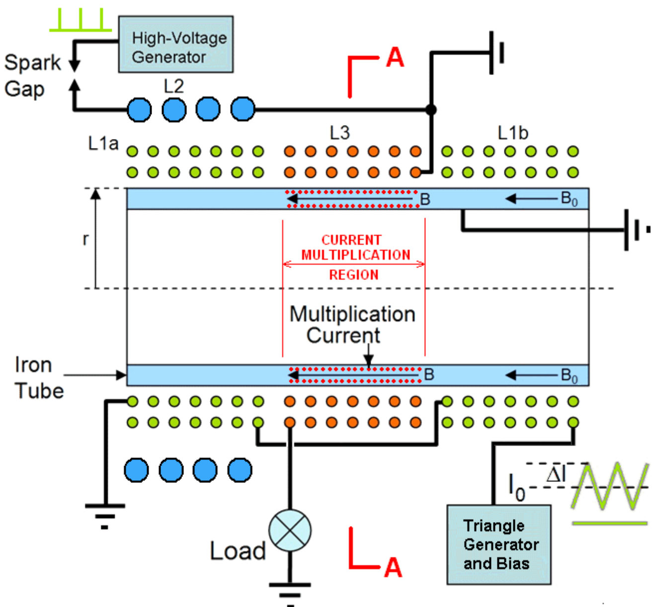
Fig.3 Iron tube based example coil. The arrangement of the coils on the tube is different in various implementations of the device. This drawing is not to scale.
