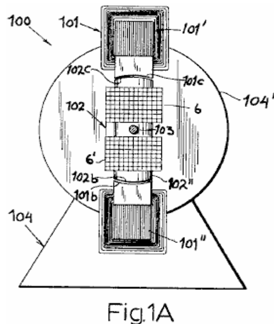
Fig.1 and Fig1A . illustrate a first embodiment of my invention, shown in axial section and in a cross-sectional view taken on line IA - IA of Fig.1 respectively.
