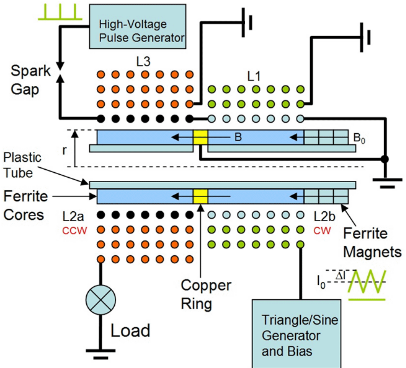
Fig.2 Cross-section of the Kapanadze-like energy device. Some of the actual implementation details may differ from the arrangement shown above, but that will not alter the operation of device. This diagram is not to scale.
